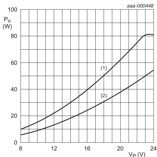
THD = 0.5 %. R_{DSon} = 0.190 \, \Omega (at T_j = 100 \, ^\circ\text{C} ), R_s = 0.05 \, \Omega , t_{w(min)} = 150 \, \text{ns} and I_{O(ocp)} = 9 \, \text{A} (typical). (1) R_L = 2 \, \Omega . (2) R_L = 4 \, \Omega .
