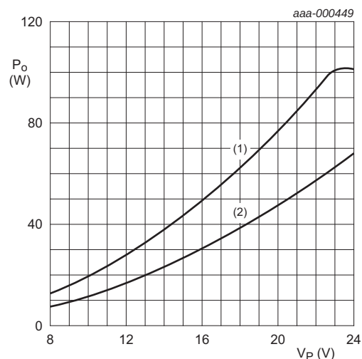
THD = 10 %. R_{DSon} = 0.190 \, \Omega (at T_j = 100 \, ^\circ\text{C} ), R_s = 0.05 \, \Omega , t_{w(min)} = 150 \, \text{ns} and I_{O(ocp)} = 9 \, \text{A} (typical). (1) R_L = 2 \, \Omega . (2) R_L = 4 \, \Omega .
